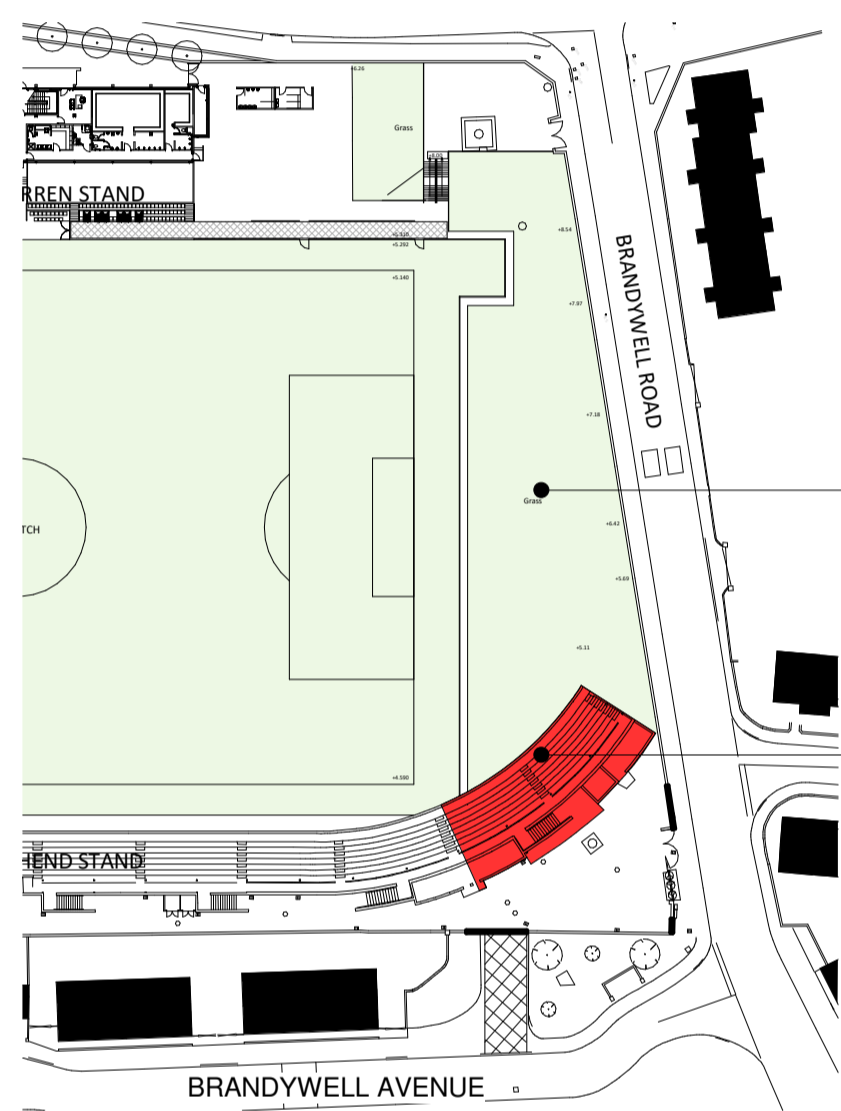
DEMOLITION PLAN
